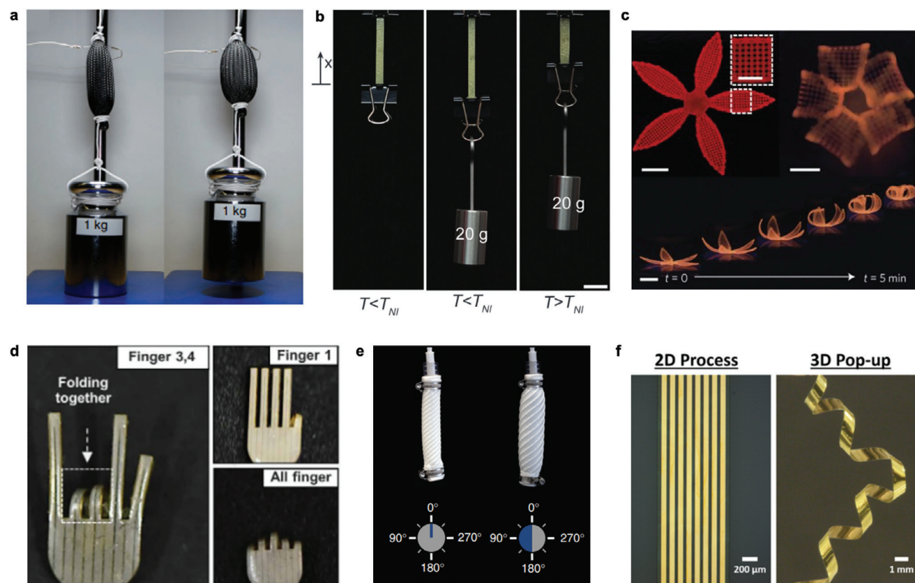
Figure 3. Examples of different motions of soft actuators. a) McKibben-type fluidic artificial muscle, composed of soft material and braided mesh sleeve, lifting weight of 1 kg through linear motion. b) Linear contractive motion by a unidirectional printed liquid crystal elastomer actuator upon heating. c) 4D printing of anisotropic hydrogels for bending actuation after swelling in water. d) Millimeter-scale soft gripper, constructed from shape memory polymer, achieving distinct finger positions through selective folding using silver nanowire Joule heaters. e) Fabricated through multimaterial 3D printing of silicones, the soft actuator exhibits a torsion motion produced by coiling stripes around the inner soft tube, set at a lead angle of 45° relative to the elongated axis. f) Liquid crystal elastomer actuator patterned with twisted nematic orientation within the substrate, undergoes controlled morphing into 3D structures, resulting from spiral motions. a) Reproduced with permission. [123] Copyright 2017, Nature Publishing Group. b) Reproduced with permission. [87] Copyright 2018, John Wiley & Sons. c) Reproduced with permission. [131] Copyright 2016, Nature Publishing Group. d) Reproduced with permission. [132] Copyright 2021, AAAS. e) Reproduced with permission. [120] Copyright 2018, Nature Publishing Group. f) Reproduced with permission. [138] Copyright 2019, American Chemical Society.
