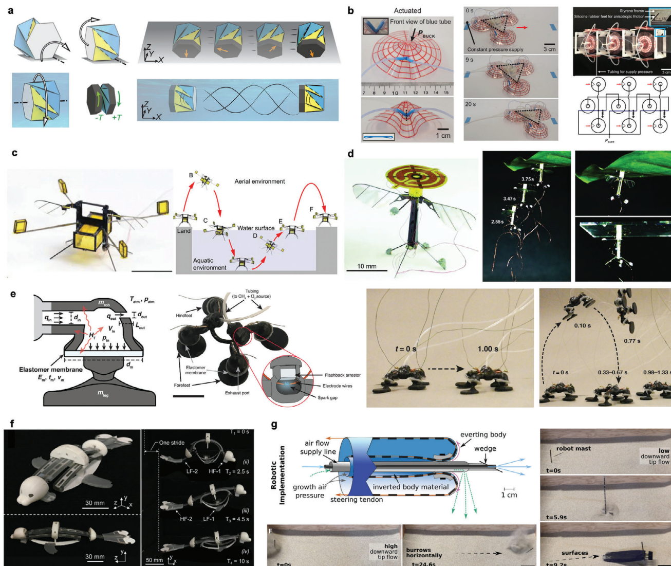
Figure 8. Multimodal locomotion by hybrid robots that use a combination of soft functional materials and rigid supports. a) Magnetically amphibious origami millirobot that can roll, flip, jump, spin, swim, and fold reversibly to pump a carried drug. b) A novel pneumatic buckling-sheet actuator used in robots that can crawl, climb a beam and dive underwater along the beam. c) Insect-scale aerial-aquatic robot that can swim and fly. d) Flying micro aerial vehicle with a switchable electroadhesive head that allows it to perch onto overhanging objects to conserve power. e) Four-legged robot that incorporates combustion microactuators for running and jumping. f) Seal-inspired amphibious robot that uses shape memory alloys to adapt to crawling on land and swimming in water. g) Soft burrowing robot made from an everting body with a pneumatically powered tip that can extend and fluidize granular media. a) Reproduced with permission. [202] Copyright 2022, Nature Publishing Group. b) Reproduced with permission. [206] Copyright 2017, AAAS. c) Reproduced with permission. [207] Copyright 2016, AAAS. d) Reproduced with permission. [203] Copyright 2022, AAAS. e) Reproduced with permission. [209] Copyright 2023, AAAS.
